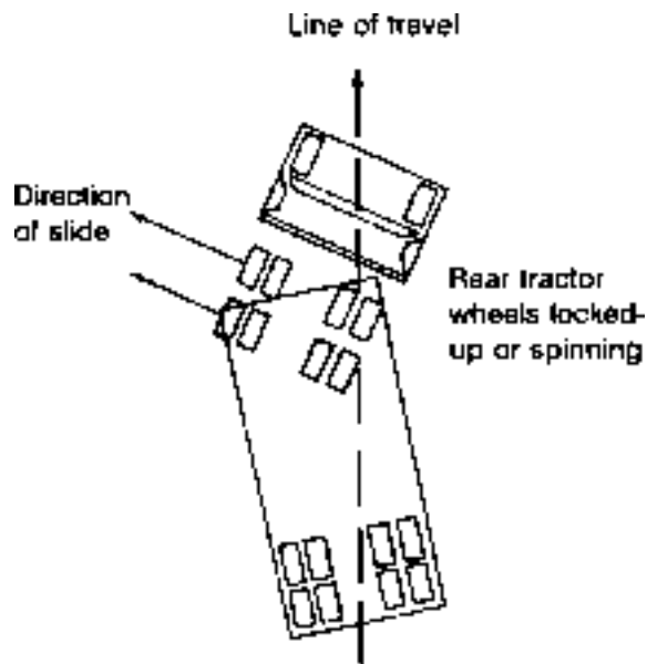
Figure 6-2 Tractor Jackknife
