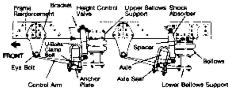
Figure 2-4 Air Suspension Parts
