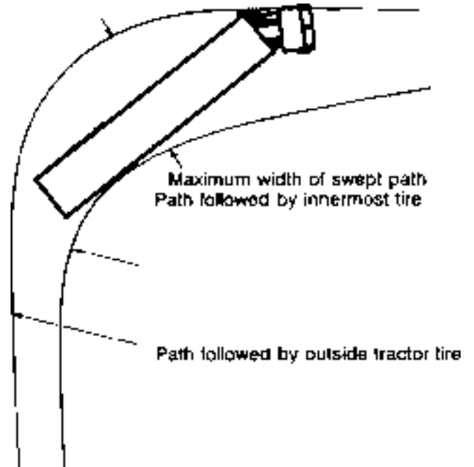
Figure 6-4 Offtracking in a 90-degree turn
