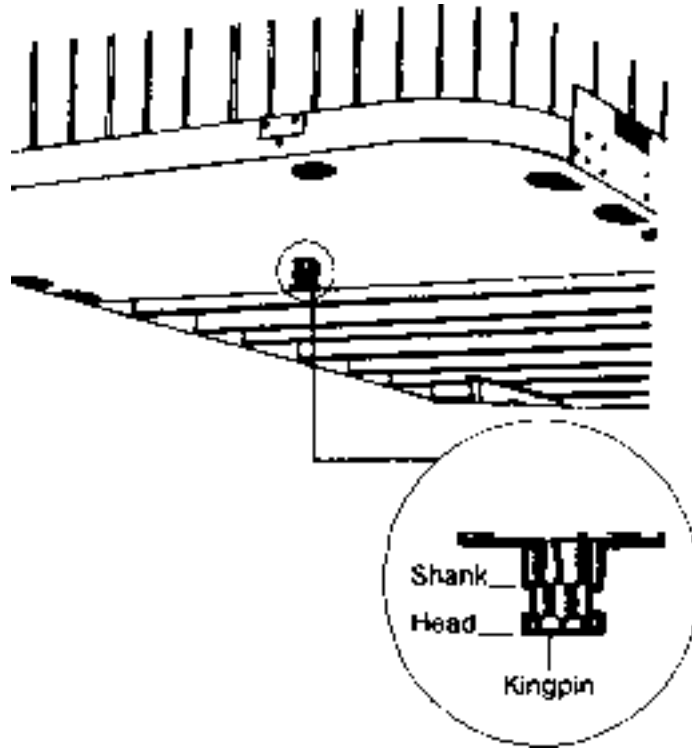
Figure 6-7 Trailer Kingpin
